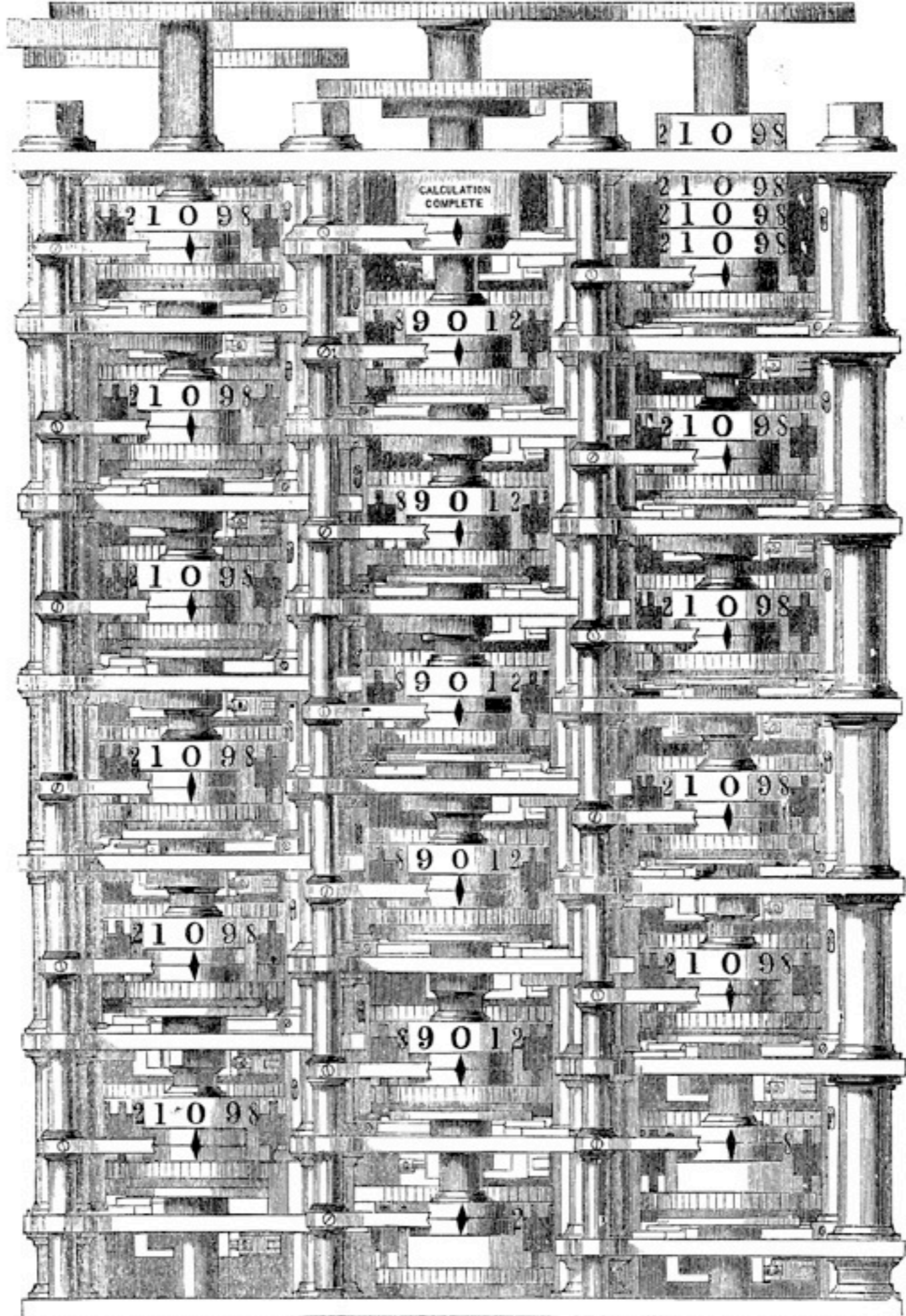
PORTION OF BABBAGE'S DIFFERENCE ENGINE.
